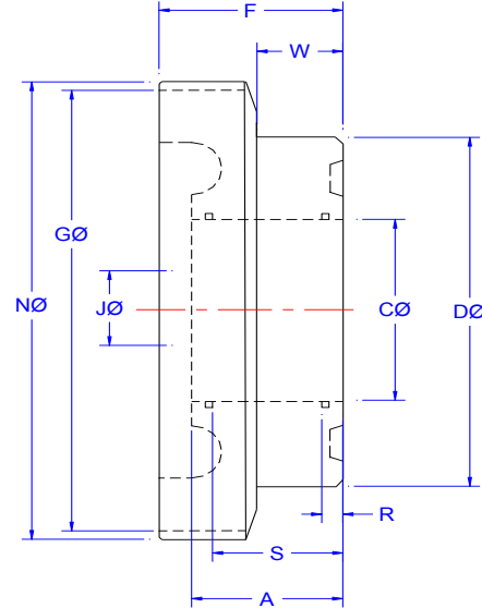
SFG120MM
